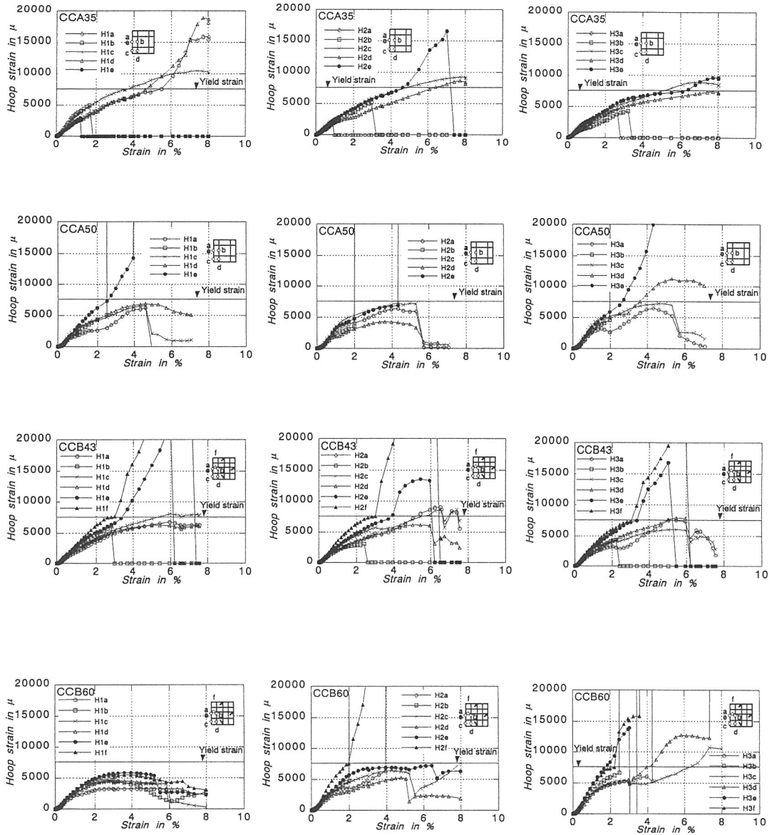
Fig. 6 Strain of lateral reinforcement
