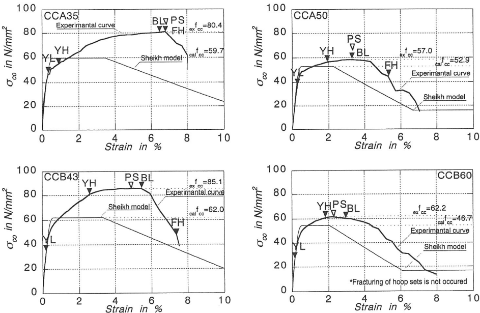
Fig.7 Comparison between the experimental curves and the model curves proposed by Sheikh
