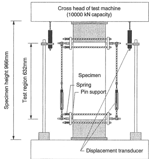
Fig. 2 Loading setup and measuring devices
