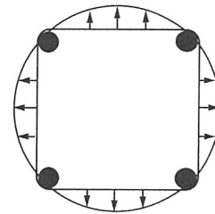
Fig.10 Lateral deformation of square column under axial compression loading
