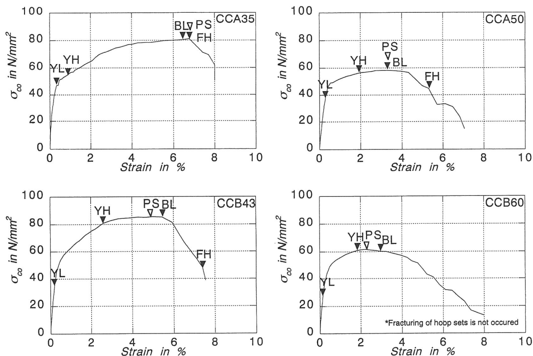
Fig. 5 Comparison of stress-strain curves
