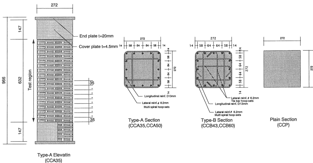
Fig. 1 Details of Test Specimens
