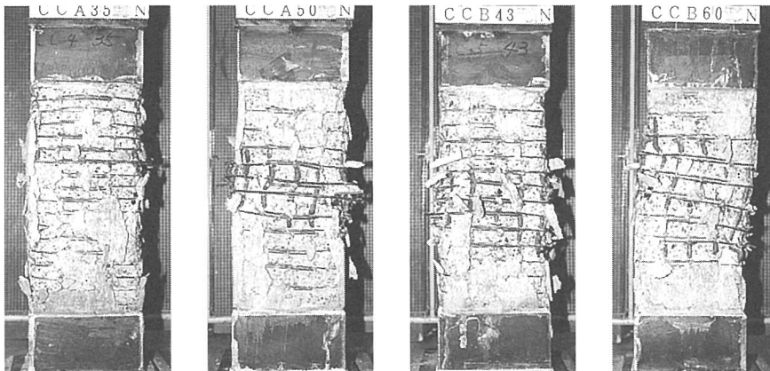
Fig. 4 Final appearance of specimens
