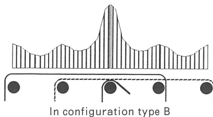
Fig.9 Assumed distributions of lateral Pressure in this test
