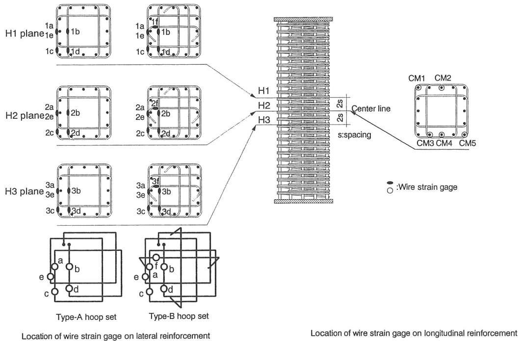
Fig. 3 Strain gages on steel reinforcement
